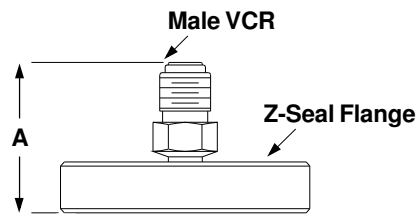
Z-SEAL TO MALE VCR FITTING
