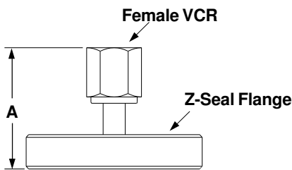
Z-SEAL TO FEMALE VCR FITTING
