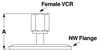
NW TO FEMALE VCR FITTING
